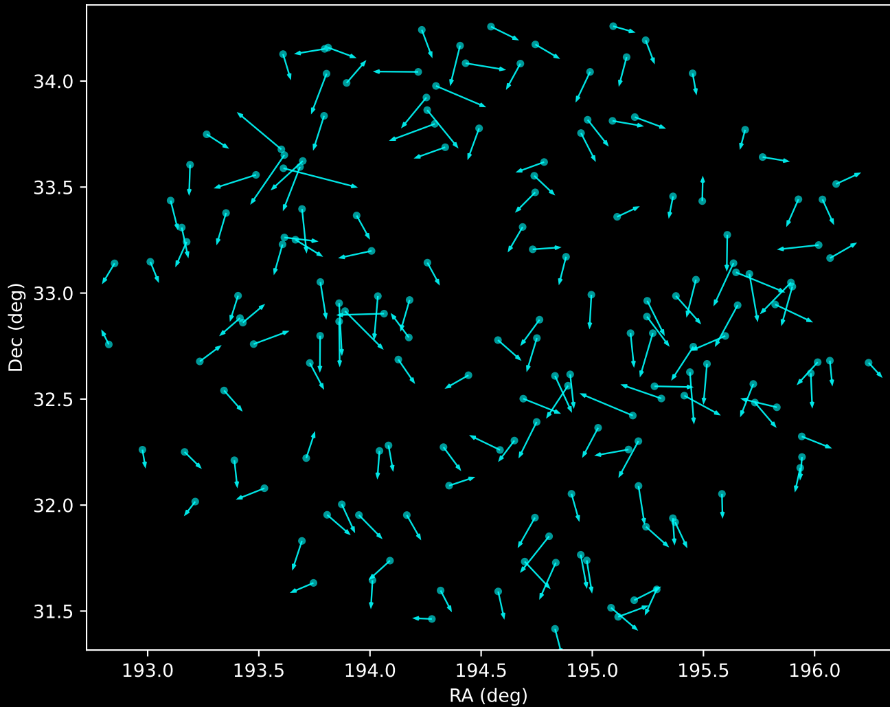
APOGEE DR17 Noise Stream Proper Motion Vectors (n=168)
