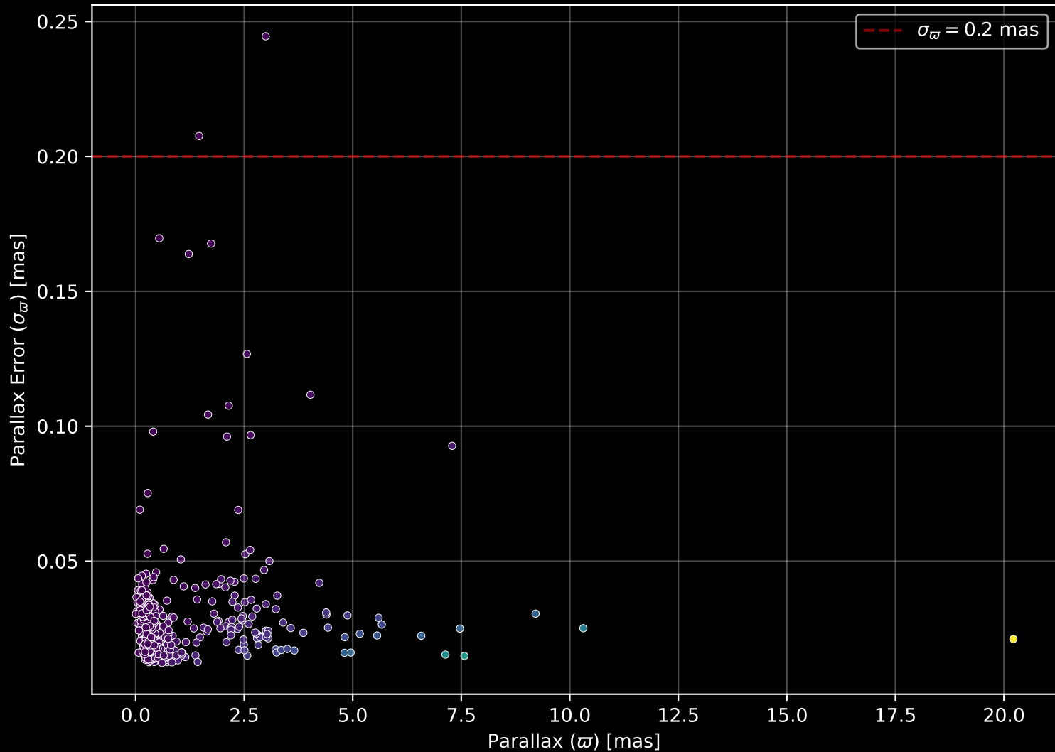
APOGEE DR17 Field: [180+08] Parallax Quality (n= 494)
