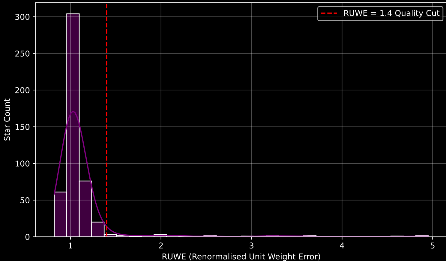
GAPOGEE DR17 Field [180+08] RUWE Distribution (n= 486)
