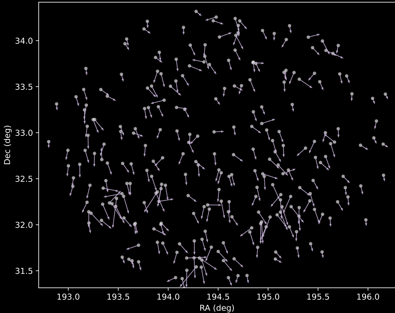
APOGEE DR17 Cluster 9 Proper Motion Vectors (n=261)
