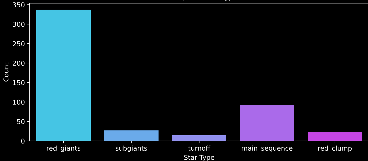
APOGEE DR17 Field: [180+08] Count plot of Star Type
