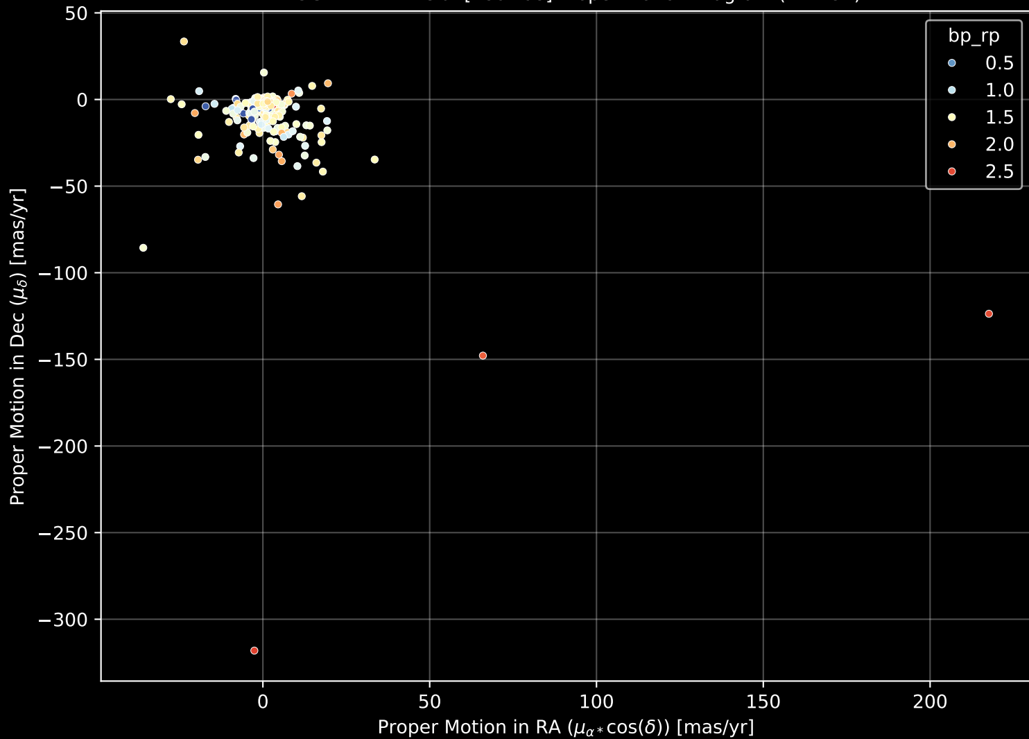
APOGEE DR17 Field: [180+08] Proper Motion Diagram (n= 494)
