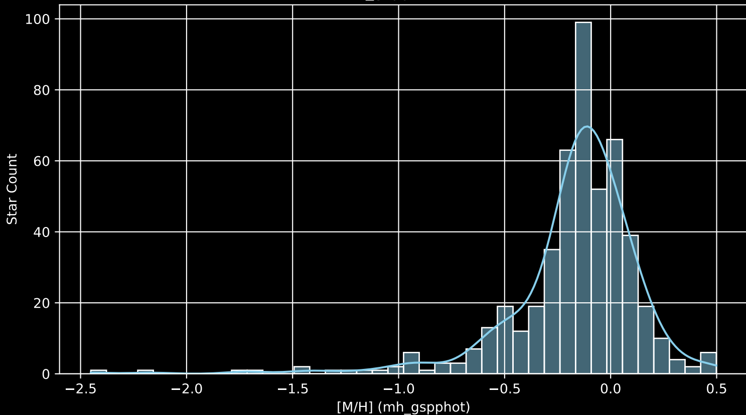
APOGEE DR17 Field: [180+08 [M/H] (mh_gspphot) (n= 490)
